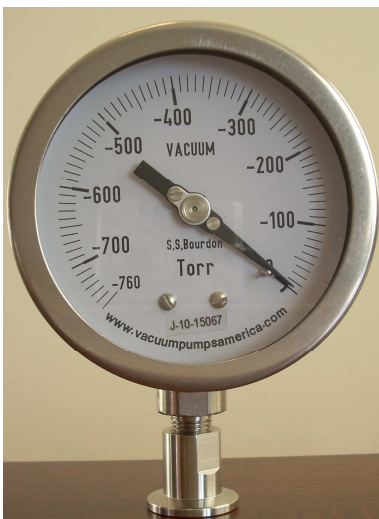
Bourdon Vacuum Gauge 0 to -760 Torr, Dry
